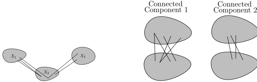
Figure 2: Every dibond is of exactly one of two possible types.
