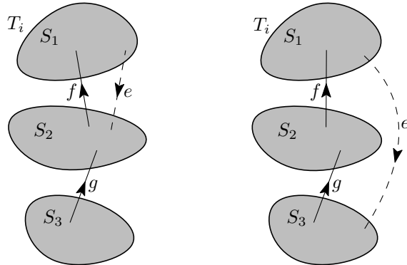
Figure 4: Figure for the proof of Proposition 4.7.
