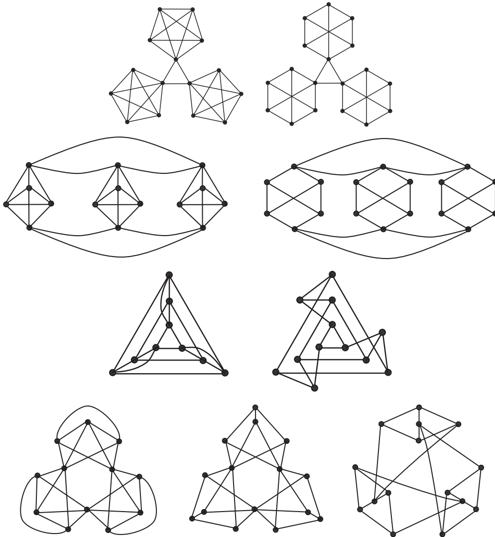
Figure 3.12. The freely \mathbb{Z}_3 -symmetric graphs derived, respectively, from the voltage graphs in Figure 3.8 with \mathbb{Z}_3 -voltages. These are minimal free obstructions for \mathbb{Z}_3 -sphericity.
