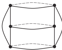
Figure 2.6. The voltage graph T_6 .
