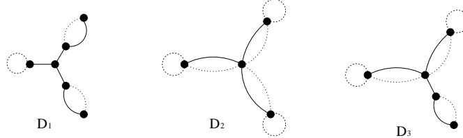
Connected excluded minors having a cut vertex with 3 bridges.
