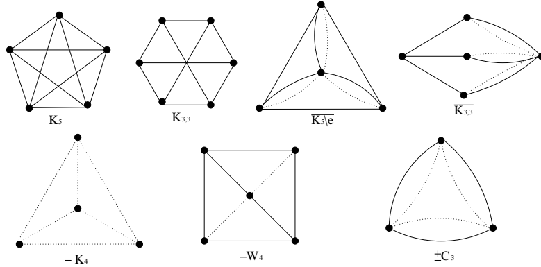
Figure 1. Excluded minors that are vertically 2-connected and jointless.
