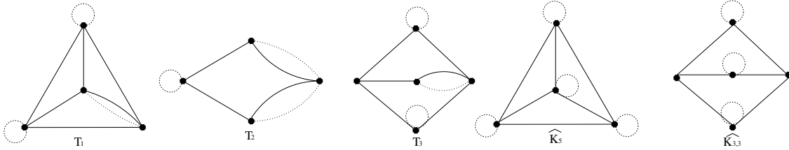
Excluded minors that are vertically 2-connected and have joints.
