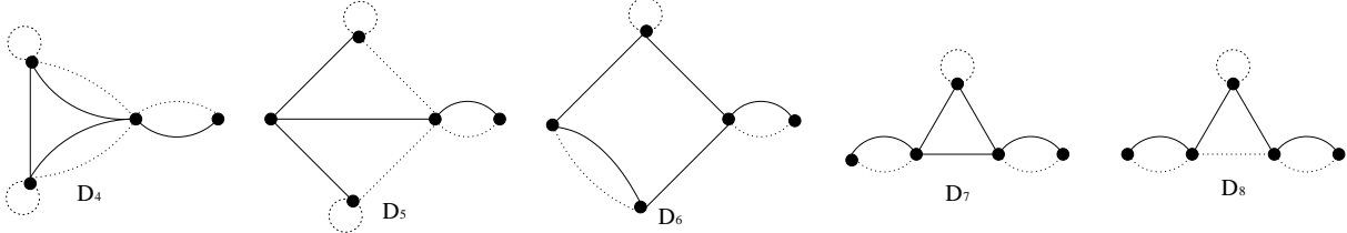
Connected excluded minors having cut vertices with at most two bridges each.
